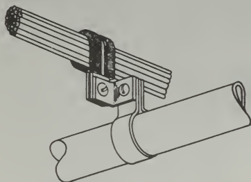
FIGURE 4-95. Separation of wires from plumbing lines.
